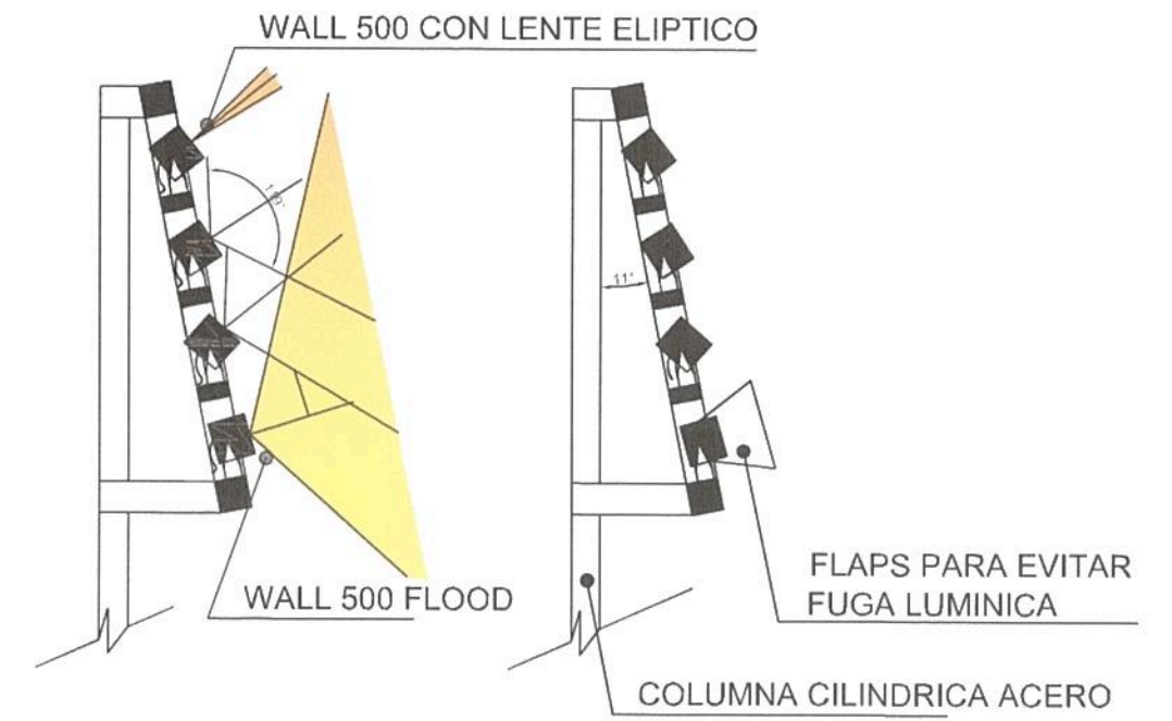
CORTE PARRILLA 4 - 8 WALL WASHER
